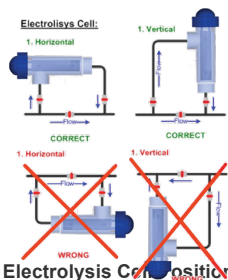
Fig 3- Electrolysis Cell Position
