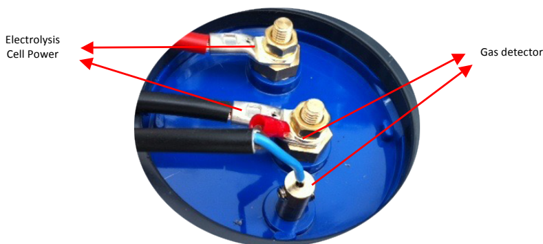
Fig 5 – Electrolysis Cell Connection Terminals
