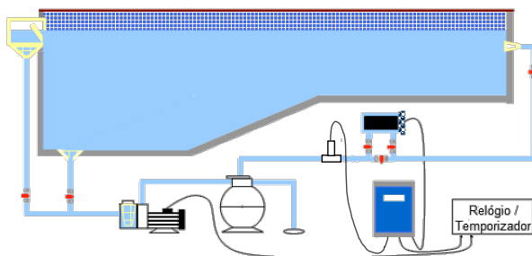
Fig 3- Hydraulic System Scheme
