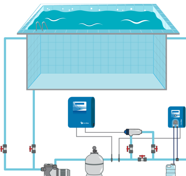
Figure 2- Hydraulique
